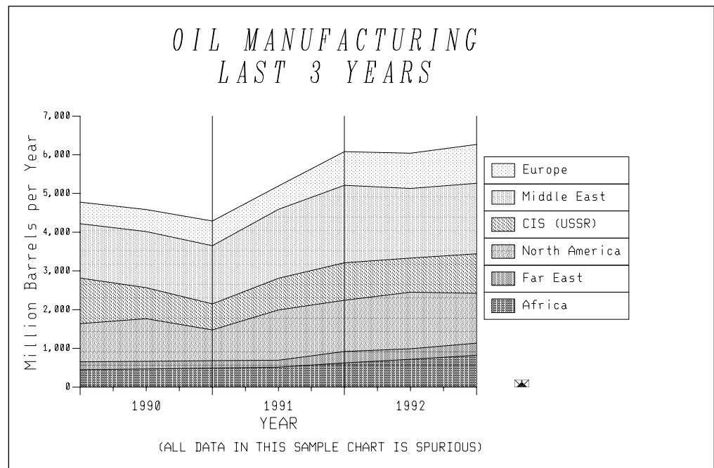
Figure 18. Surface chart
