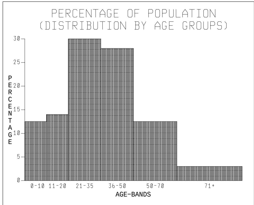
Figure 19. Histogram
