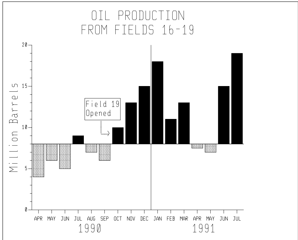
Figure 22. Bar chart
