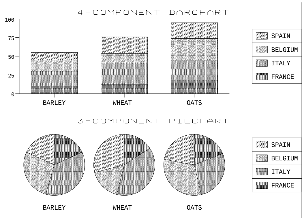
Figure 26. Comparison of composite bar chart with multiple pie chart
