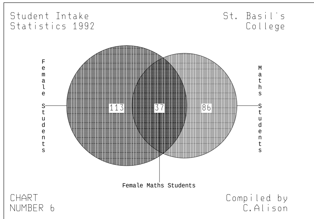
Figure 28. Venn diagram
