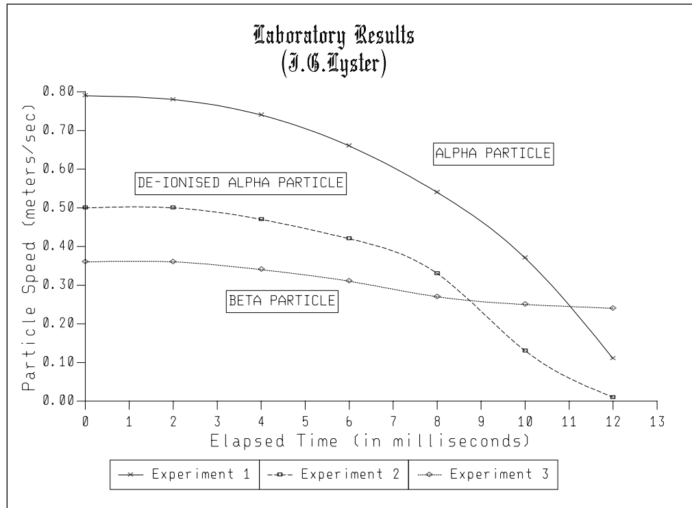
Figure 15. Line graph (with curve fitting)
