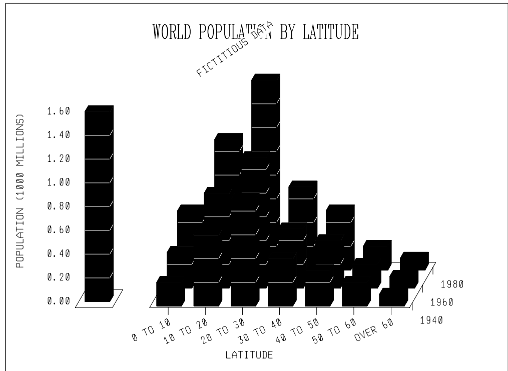
Figure 23. Tower chart
